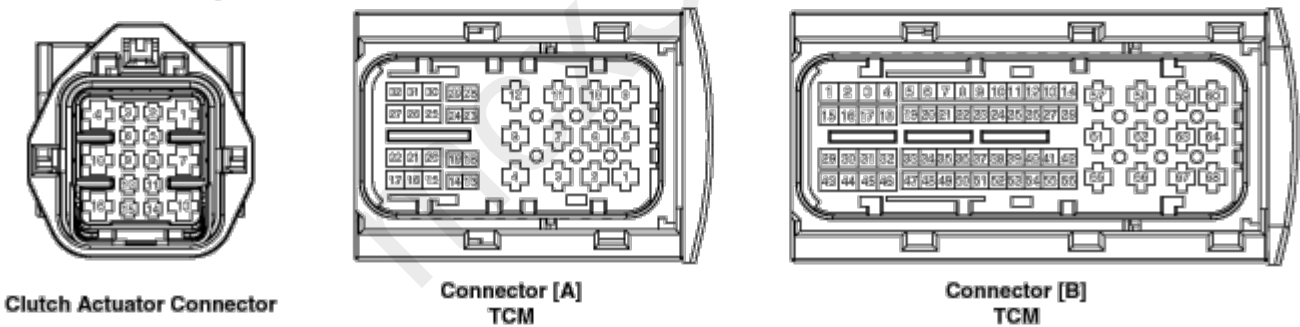
[Harness Connector]
